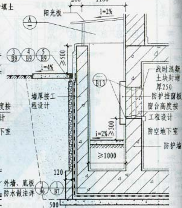
③ 挡板式窗井
