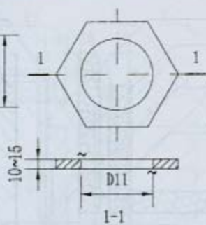
2 止水环
