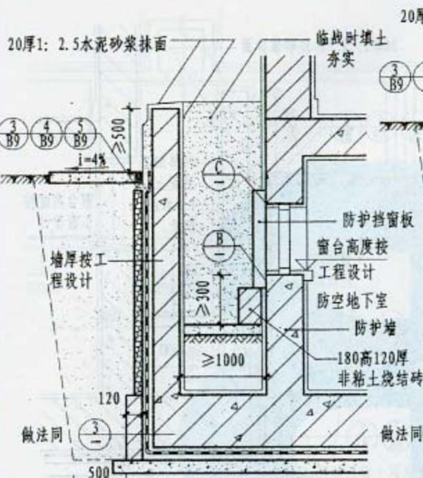
① 战时全填土窗井
